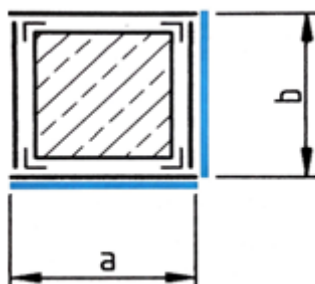
Figure 65: Poteau ; A = 2 * (a+b) * h
