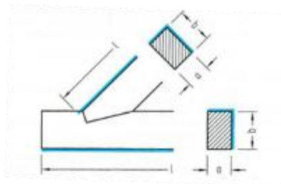
Figure 1: plus grande longueur = l , section totale = a \times b
