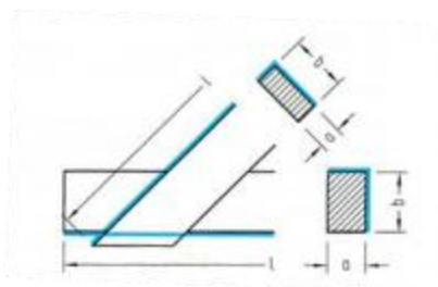
Figure 2: plus grande longueur = l , section totale = a \times b
