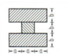
Figure 11: section totale = 7 \times a \times b
